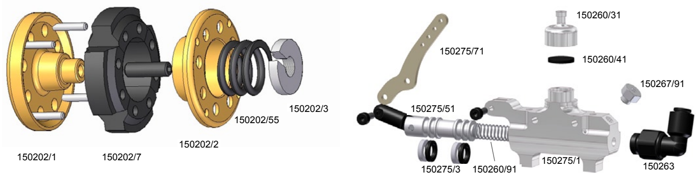
150275 Kit Master cylinder 10mm
