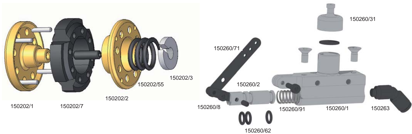
150260 Kit Master cylinder
