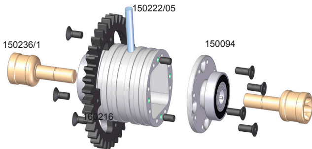
150222 Kit Diferential
