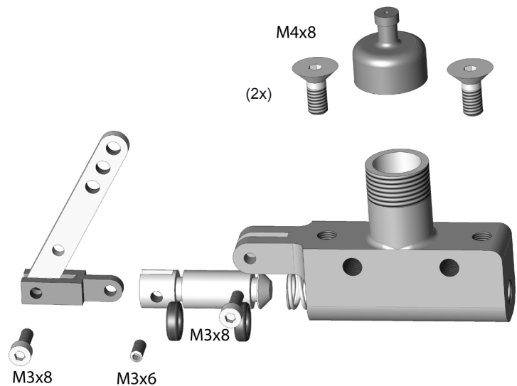
Rear brake
