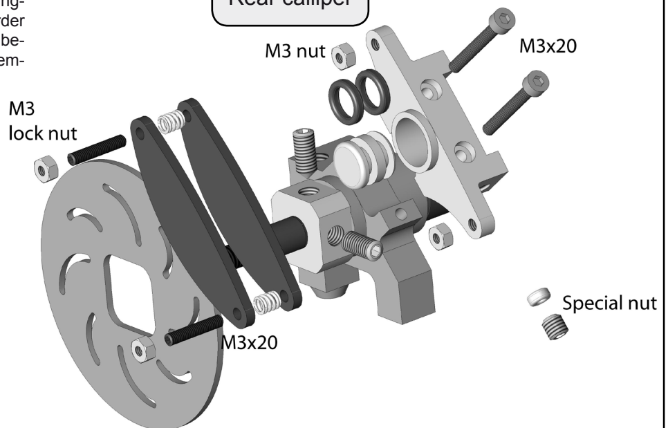
Rear calliper
