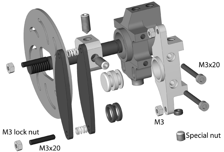
Rear calliper
