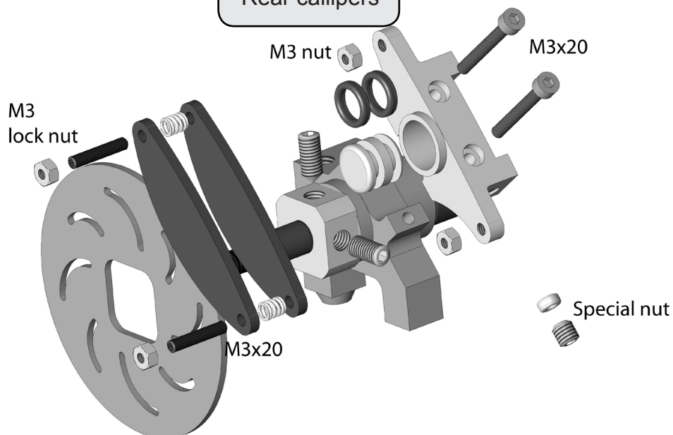
Rear callipers
