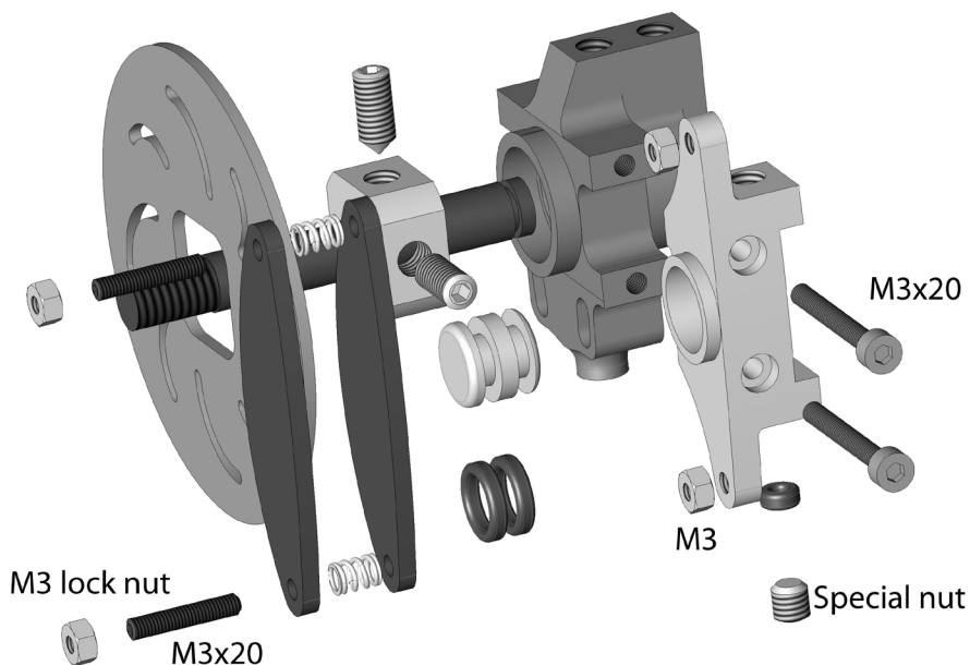
Rear callipers
